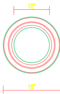
ROUND BASE
